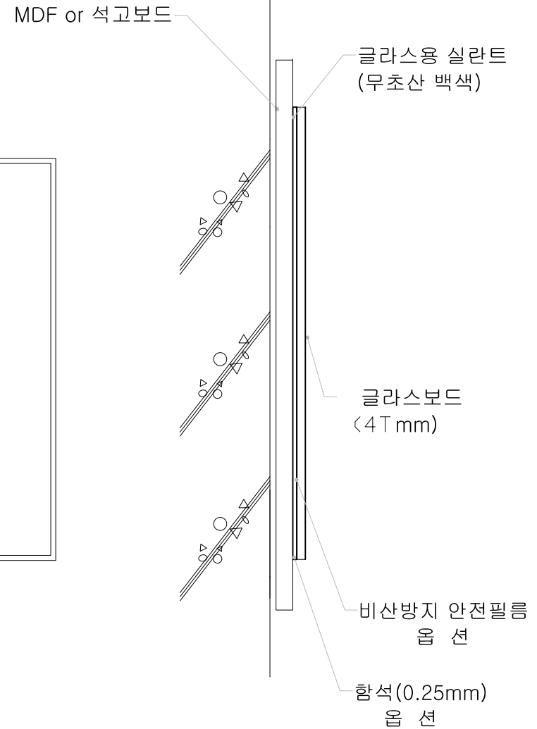
SIDE VIEW SCALE NONE
